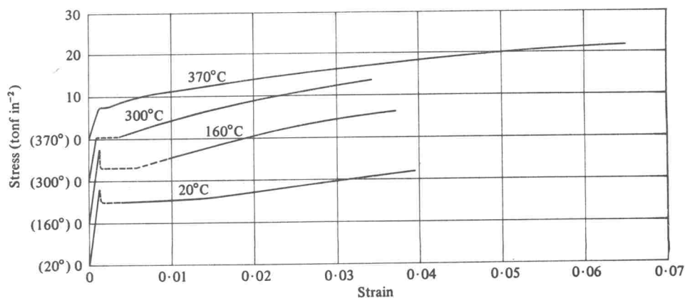
Figure 15. Tension tests on mild steel EN3A.
